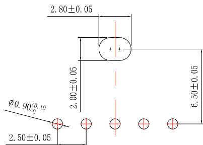
Recommend P. C. B Layout
