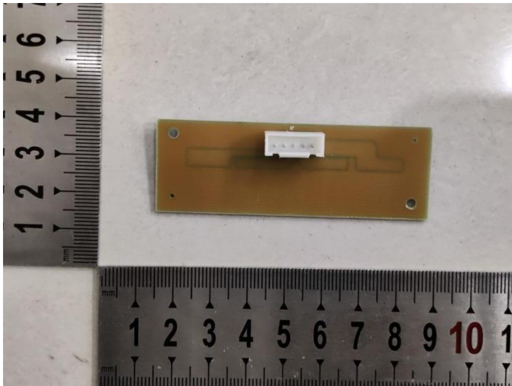
Figure 10.PCB view
