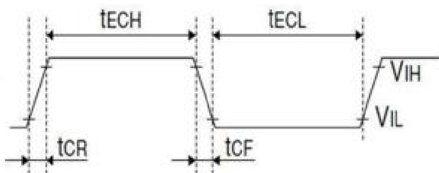
Figure: UK39-F high precision receiver UART timing specifications
